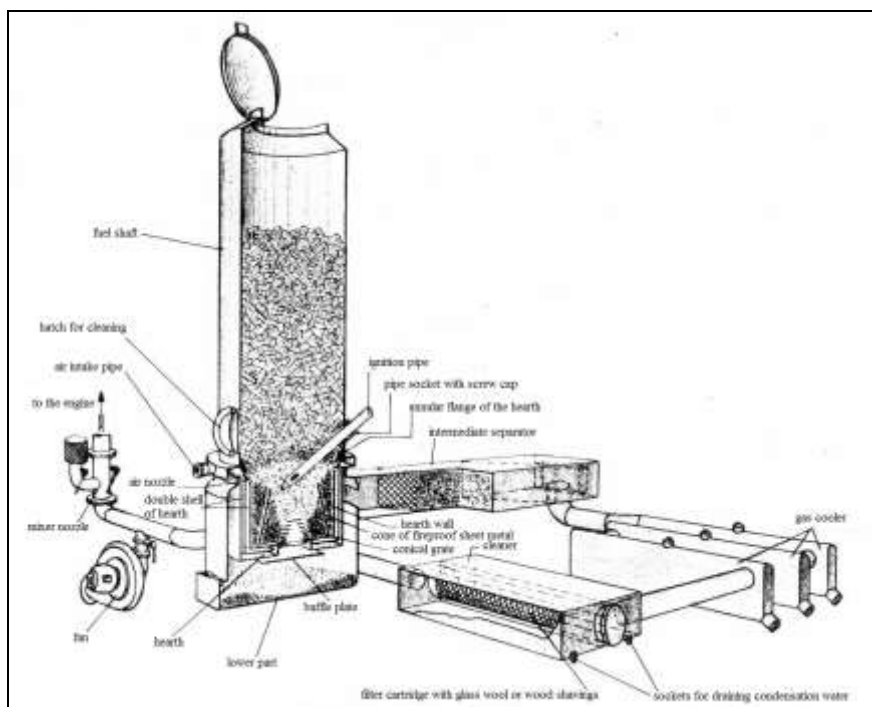
Illustration 11: Design of an Ostmark producer gas generator. (Berg 2019, p. 468; descriptions translated)
