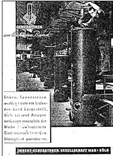
Ill. 131: The Imbert Generator was the most common wood-gas generator of the Third Reich, here during its mass production on a conveyor belt in Cologne during 1943. ( Motortechnische Zeitschrift , no. 6/7, 1943, p. 3A.)
