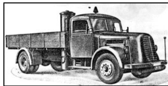
III. 132: The Austro-Fiat 4 D 90 A, manufactured with wood-burning gas generator.
