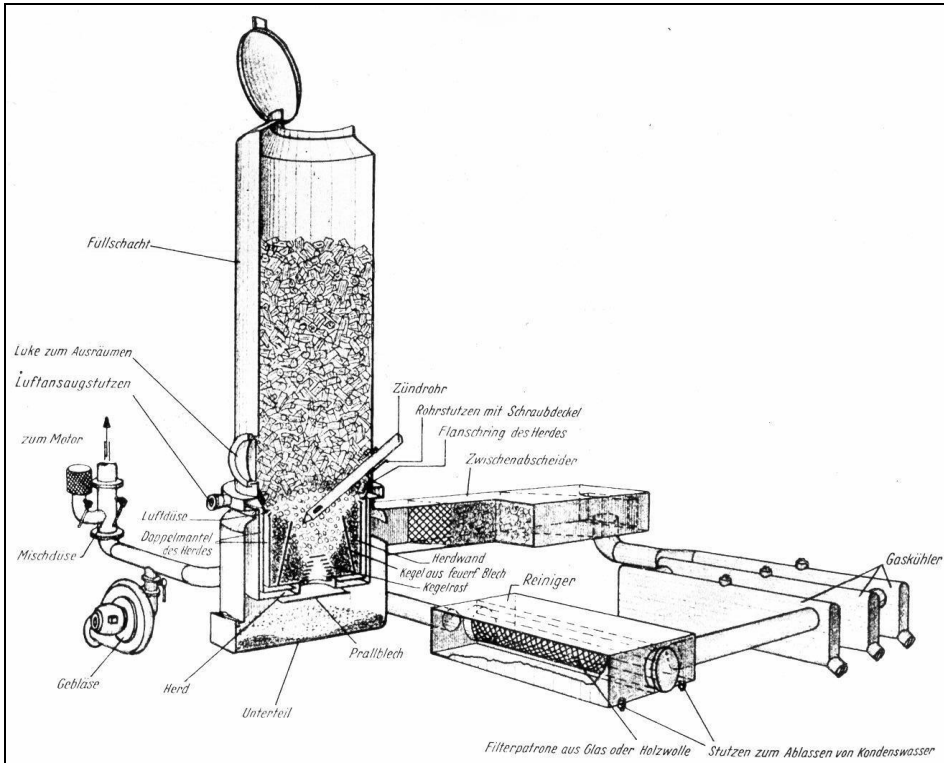
III. 134: Design of an Ostmark Gas Generator.
